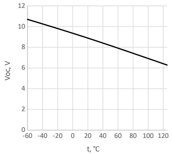
Pic. 2 – V_{oc} vs temperature
